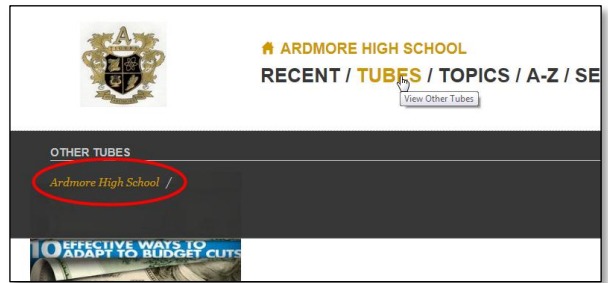
SupeTube Server
